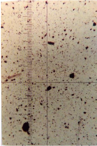
ISO 23/21/18 NAS 12
