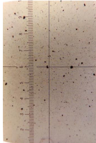
ISO 21/19/16 NAS 10
